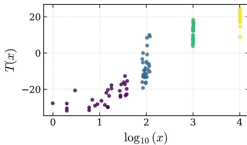
Falcon-RW-7B
